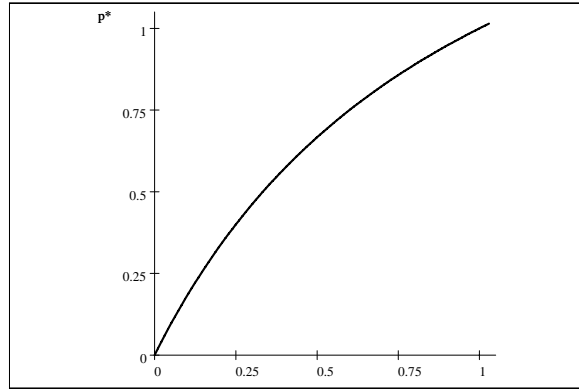
Threshold p^*(x)
